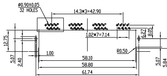
RECOMMENDED PC BOARD LAYOUT AS VIEWED FROM COMPONENT SIDE TOLERANCE \pm 0.05\text{mm}
