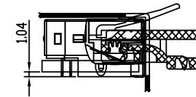
A-A SIDE VIEW SHOWING WITH PLUG
