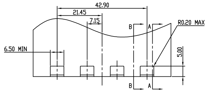
RECOMMENDED PANEL LAYOUT
