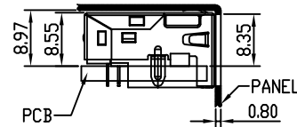
B-B SIDE VIEW SHOWING WITH PANEL AND PCB
